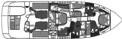
Three Stateroom Layout
